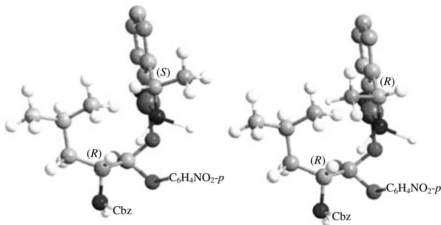
Possible mutual orientations of the \alpha -methyl fragment in the R and S isomers of complex I and the side-chain substituent in the ( R )-leucine derivatives in the transition state for the hydrolysis of the ester group.
